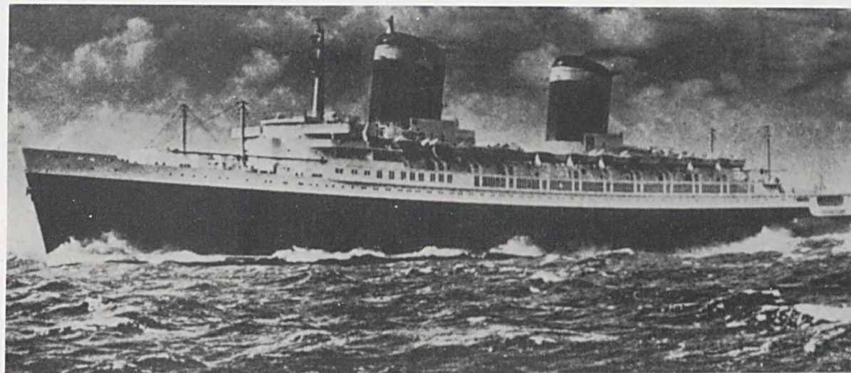
he S.S. United States . The largest merchant ship ever built in America. Keel laid February 8, 1950. Christened June 1951. Principal characteristics—Length overall 990 feet. Beam 101 feet 6 inches. Depth, Keel to top of superstructure 122 feet. Number of decks 12. Propulsion: Steam Turbine, quadruple screw. Speed 30 knots. Gross Tonnage 53,330. Net Tonnage 28,000.
